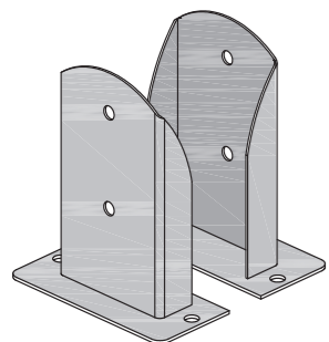
PORTAPILASTRI NEW103
